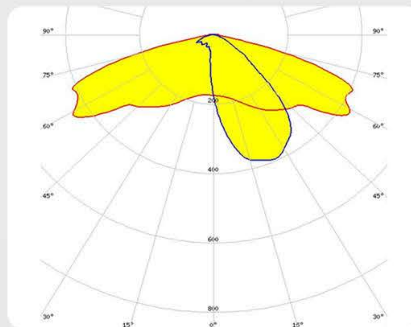
LIGHT DISTRIBUTION CURVE
