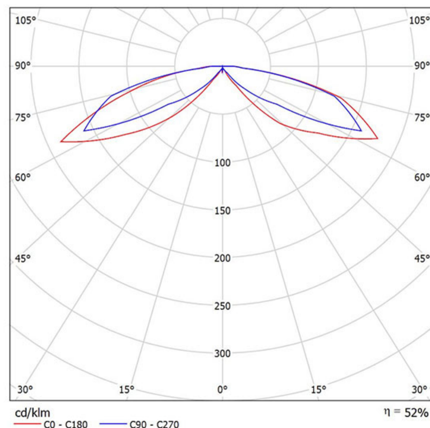
LIGHT DISTRIBUTION CURVE
